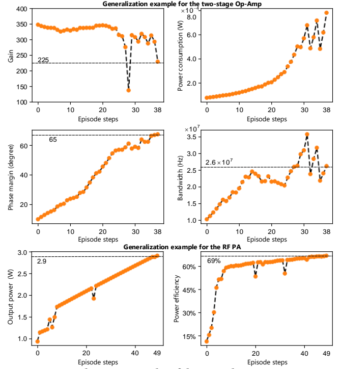
Figure 6: Generalization examples of the trained RL agent attempting to reach one group of the unseen specifications for each circuit.
