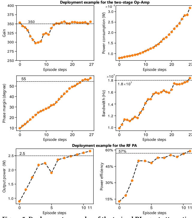
Figure 5: Deployment examples of the trained RL agent attempting to reach one group of the target specifications for each circuit.
